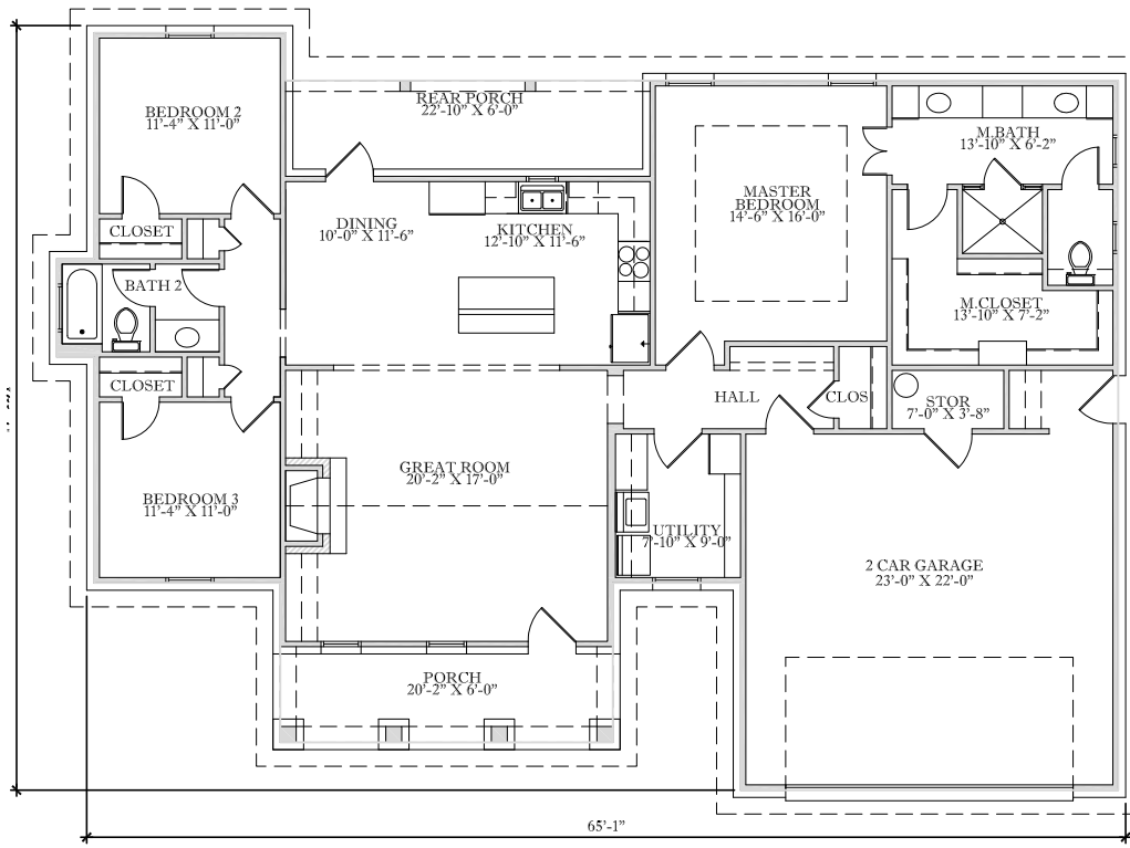
MAIN FLOOR
