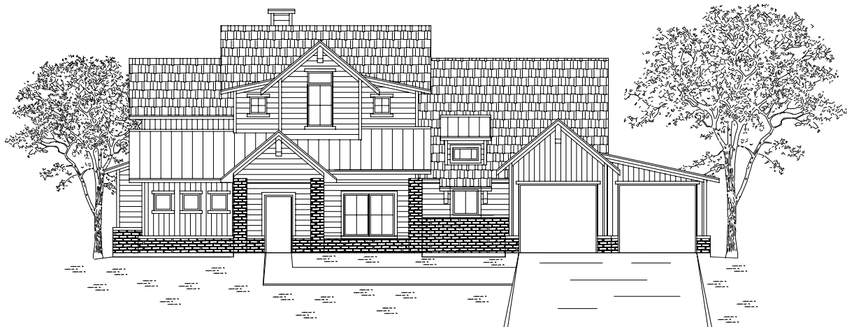
FRONT ELEVATION - OPT. B
