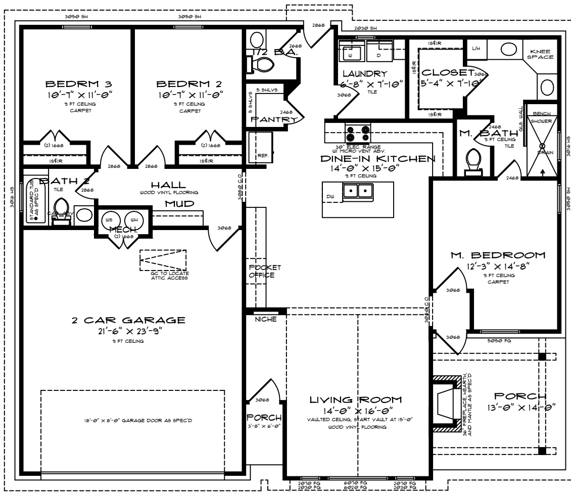
FLOOR PLAN
