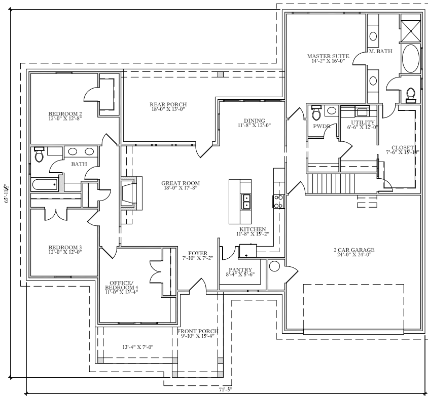
MAIN FLOOR
